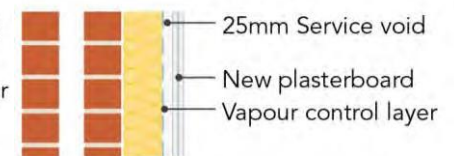
Internally insulated brick cavity
