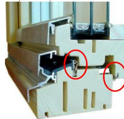
Triple glazed opening sash – timber frame with aluminium cladding and two seals (Source: Internorm)
