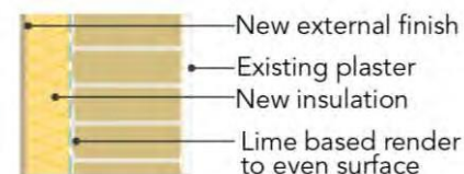
Externally insulated Stone Wall
