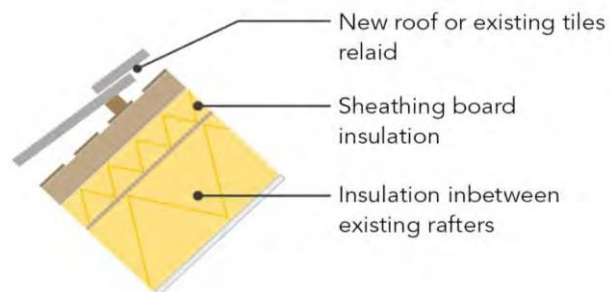
Rafter insulation detail
