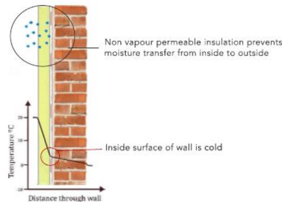
The risk of condensation with internal insulation
