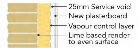
Internally insulated Stone Wall
